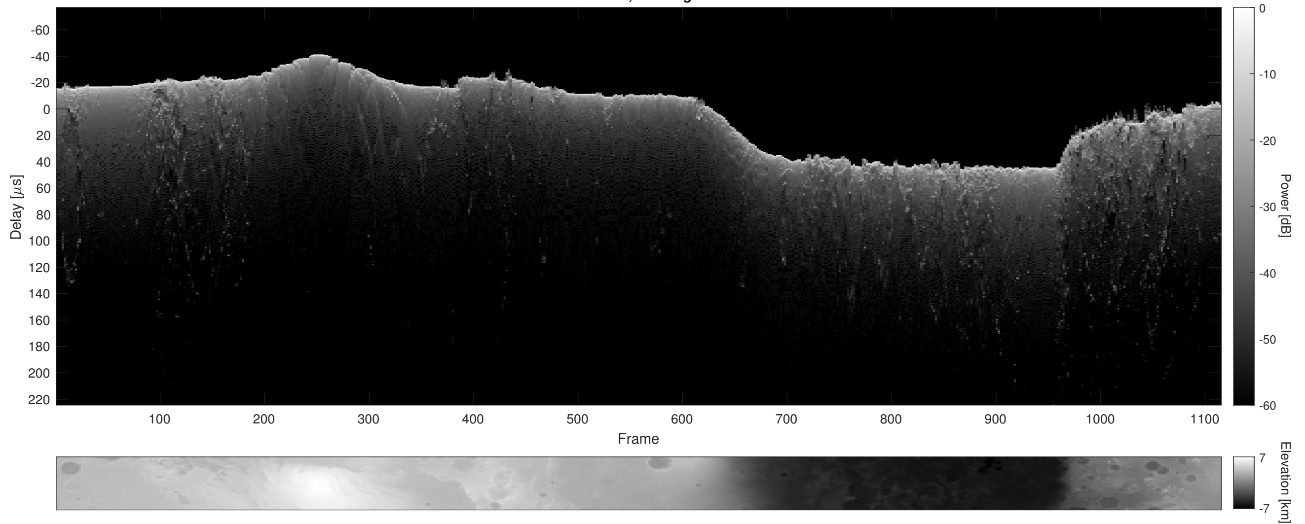
Orbit 2404, Cluttergram
