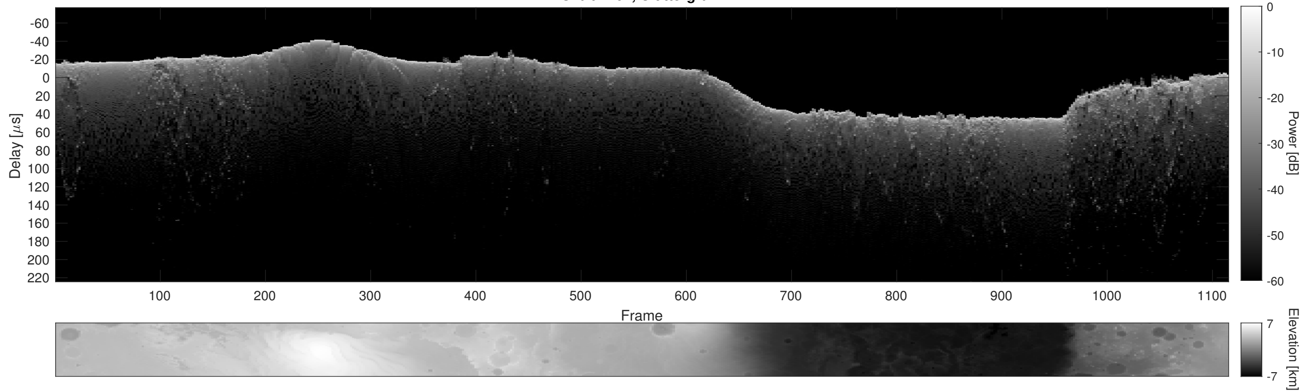
Orbit 2404, Cluttergram
