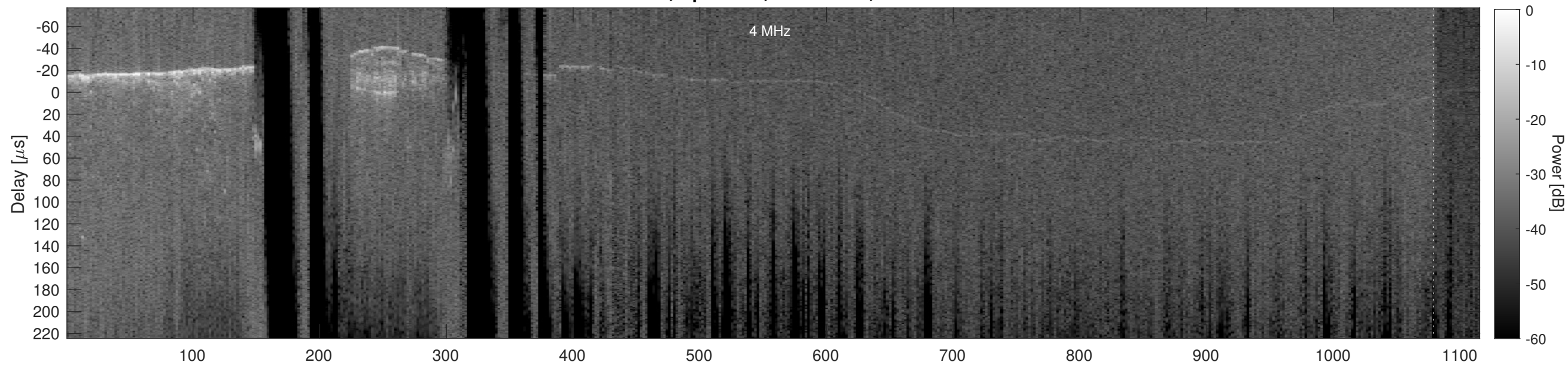
Orbit 2404, Cluttergram
