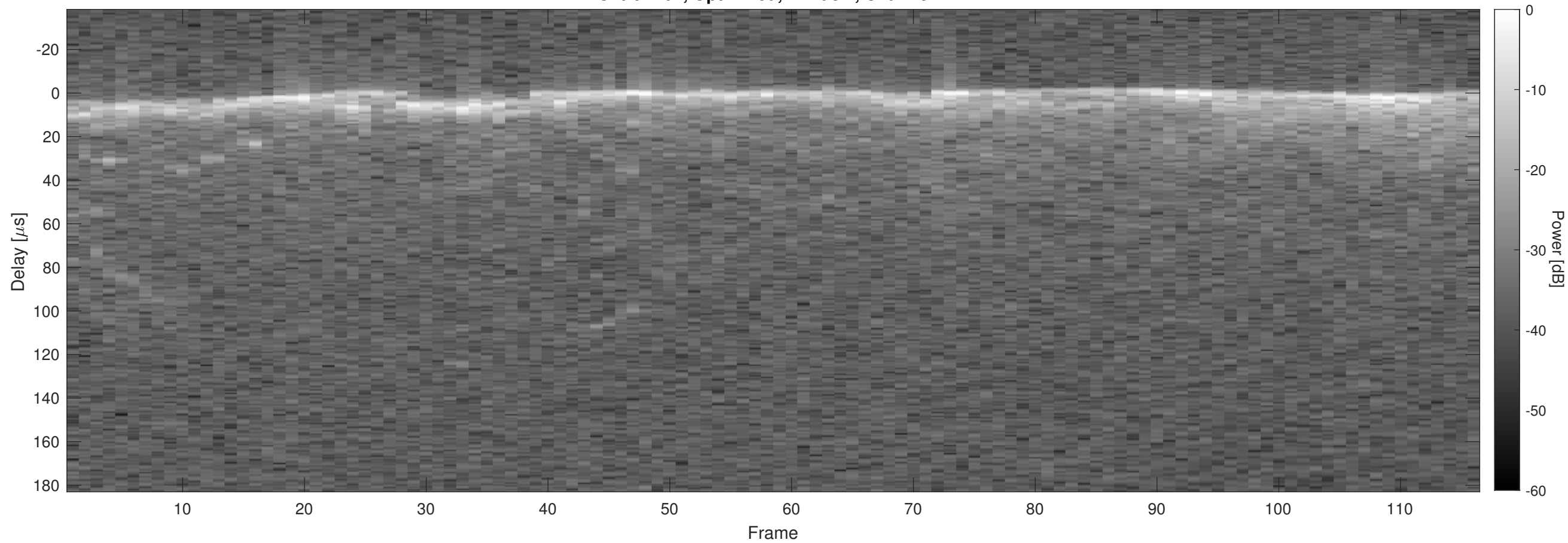
Orbit 2407, Optimized, Window, Channel 2
