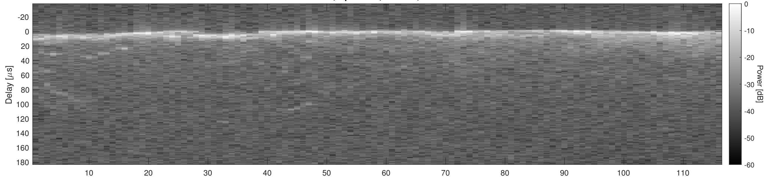
Orbit 2407, Optimized, Window, Channel 2
