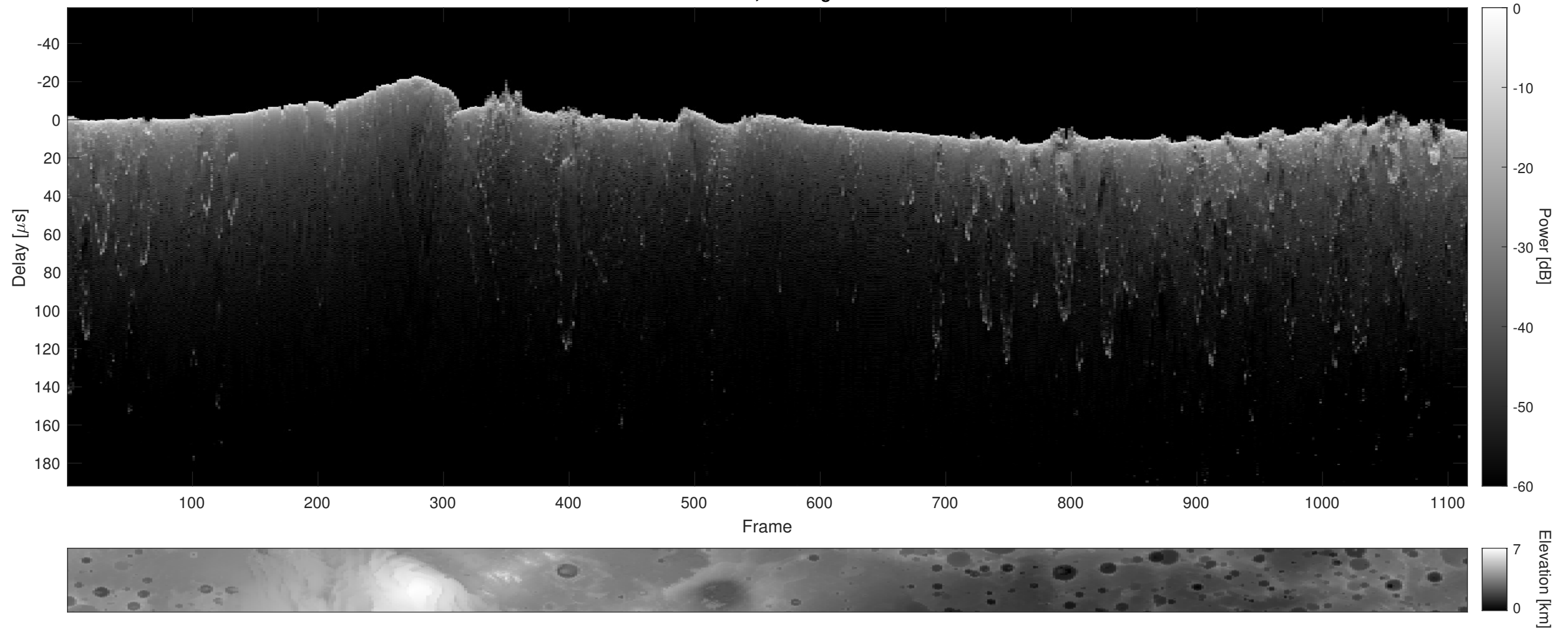
Orbit 2408, Cluttergram
