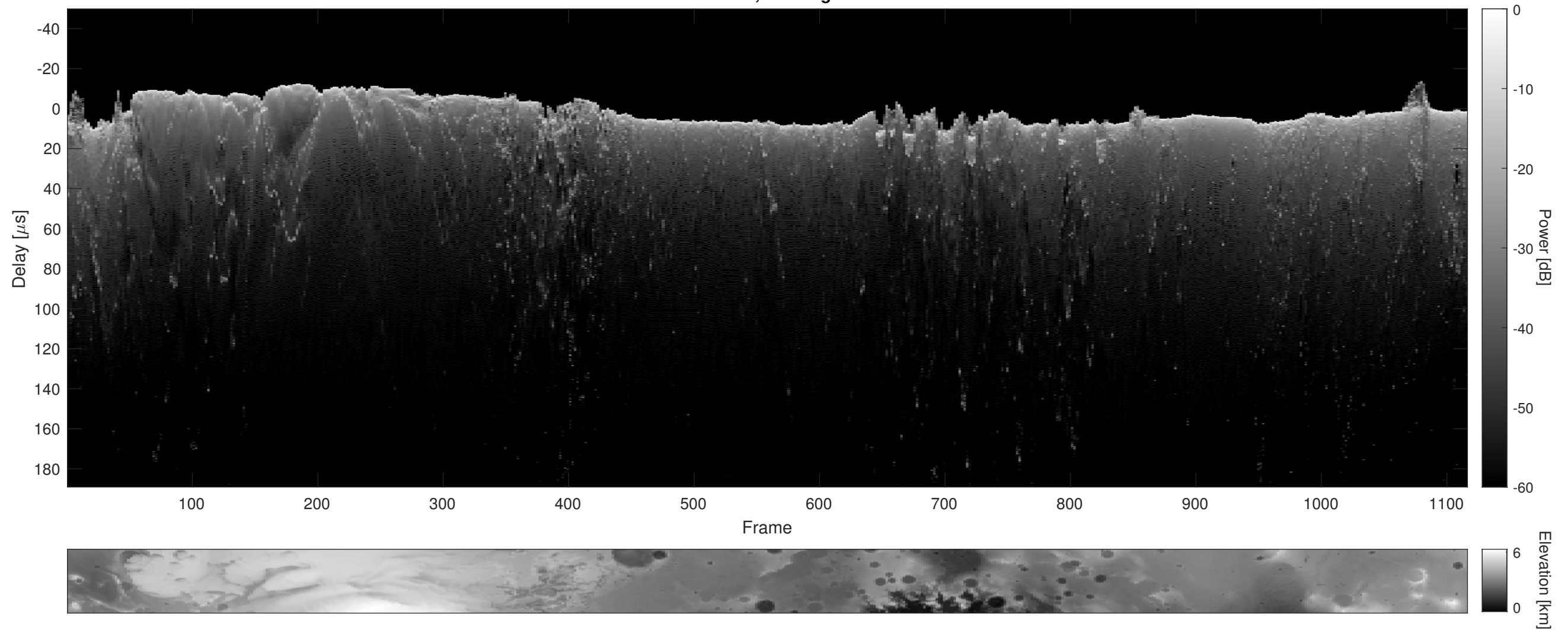
Orbit 2409, Cluttergram
