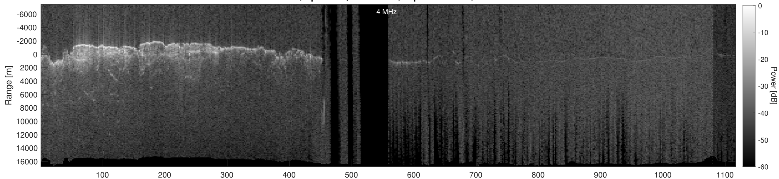
Orbit 2409, Depth-Corrected Cluttergram
