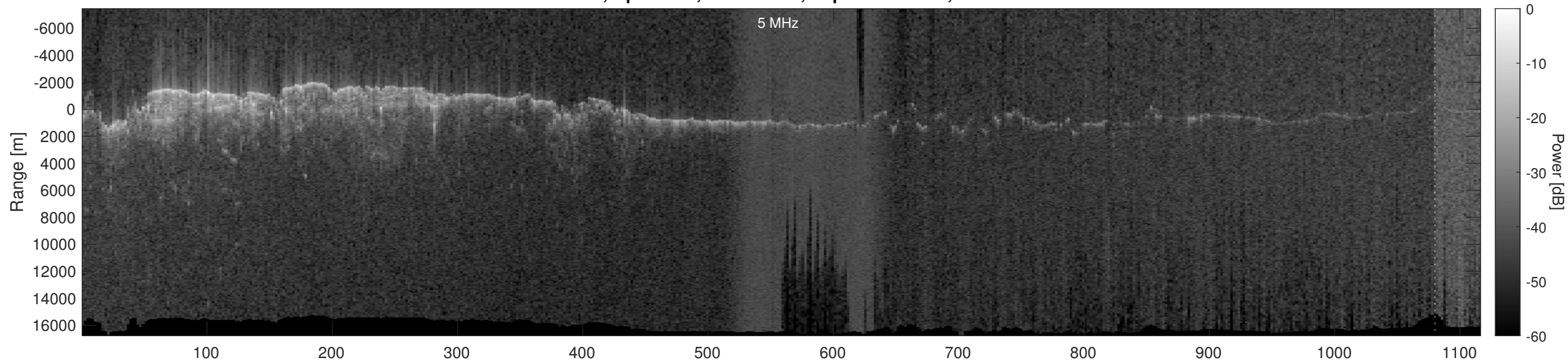
Orbit 2409, Optimized, No Window, Depth-Corrected, Channel 2
