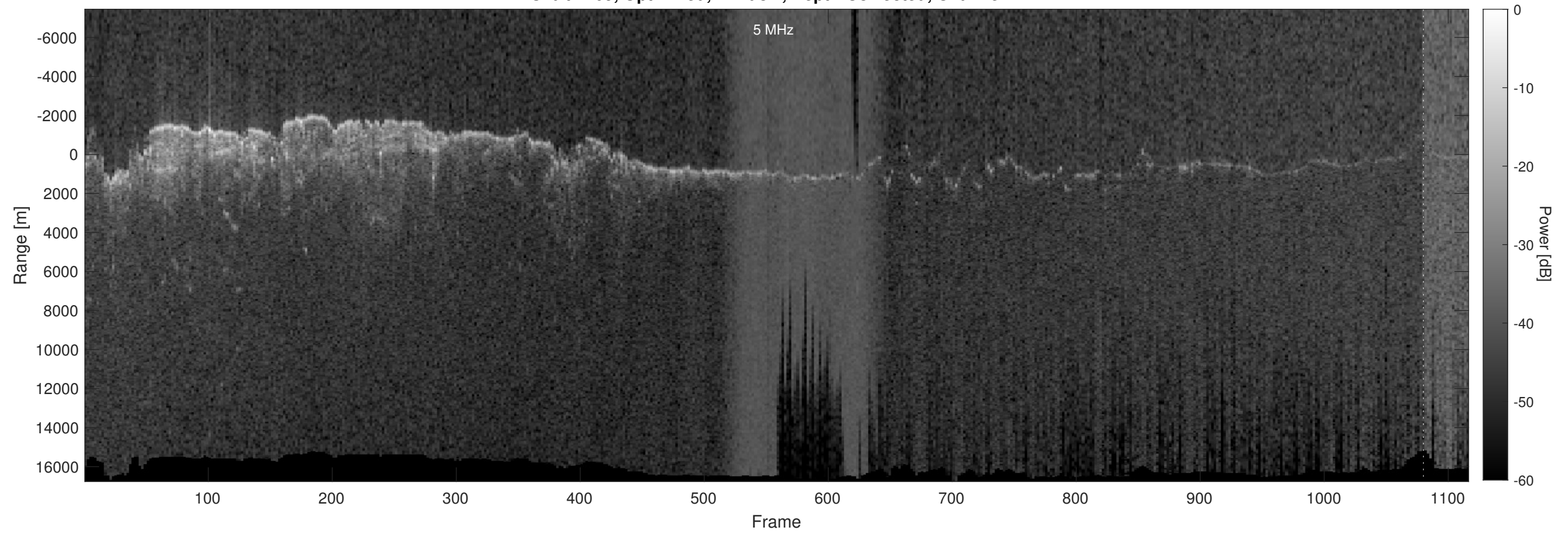
Orbit 2409, Optimized, Window, Depth-Corrected, Channel 2
