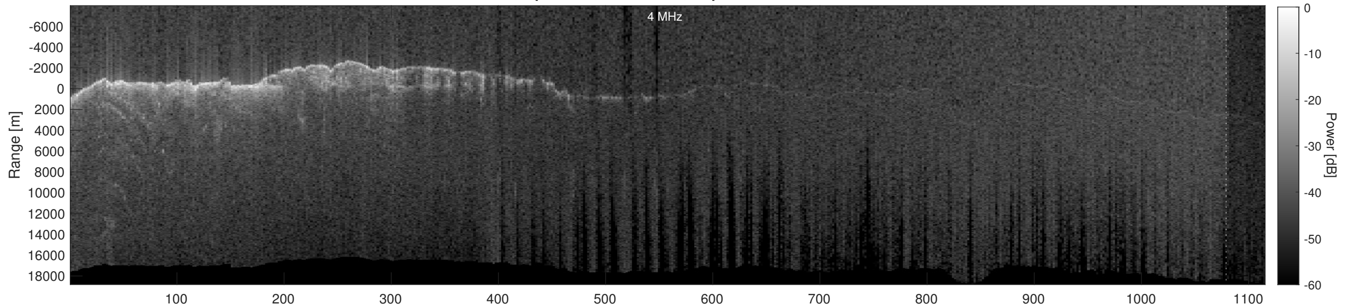
Orbit 2410, Depth-Corrected Cluttergram
