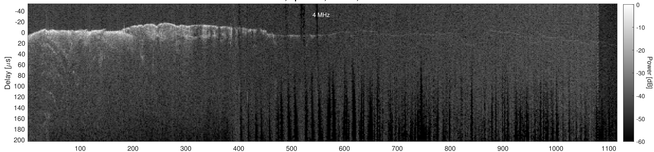
Orbit 2410, Cluttergram
