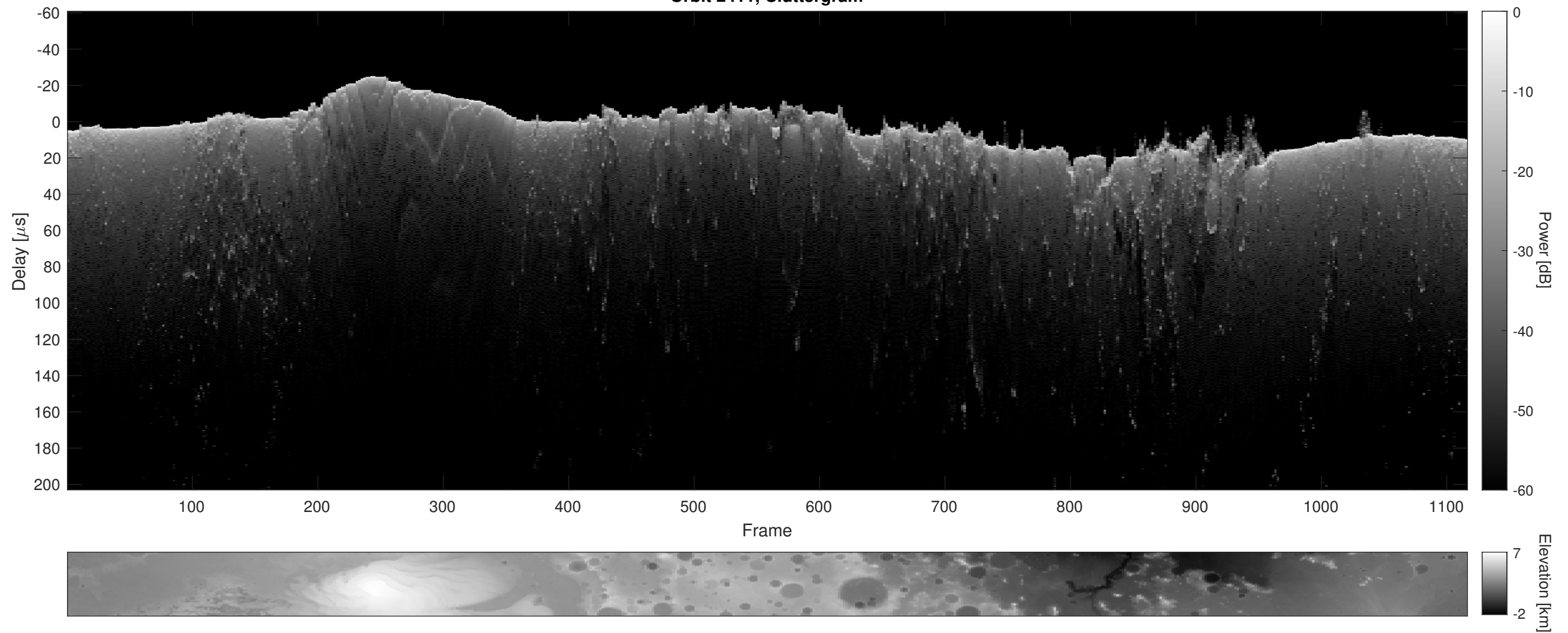
Orbit 2411, Cluttergram
