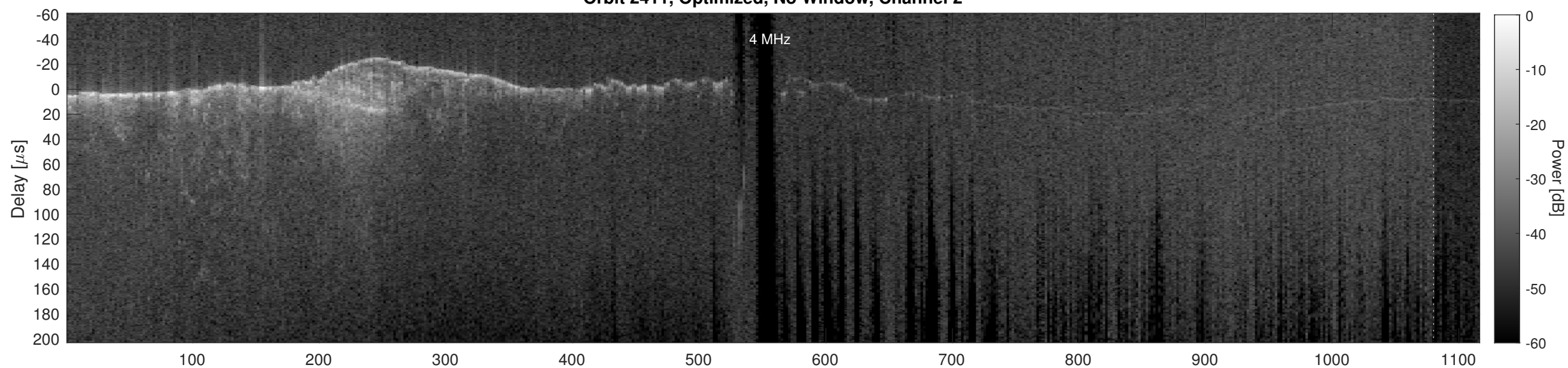
Orbit 2411, Cluttergram
