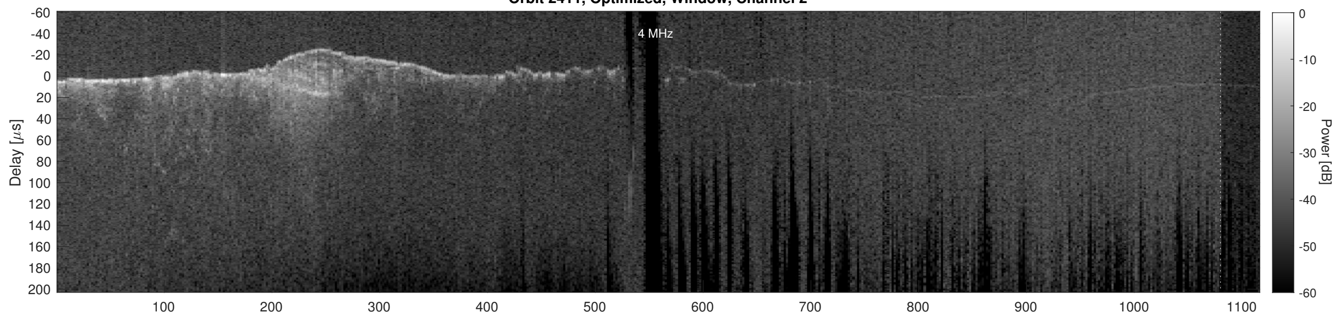
Orbit 2411, Cluttergram
