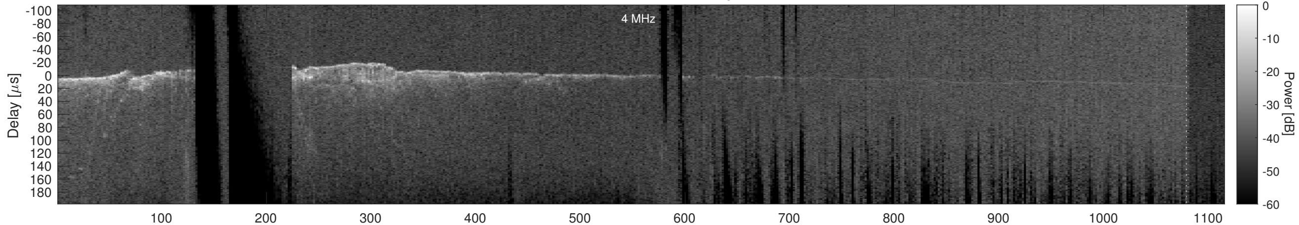
Orbit 2412, Cluttergram
