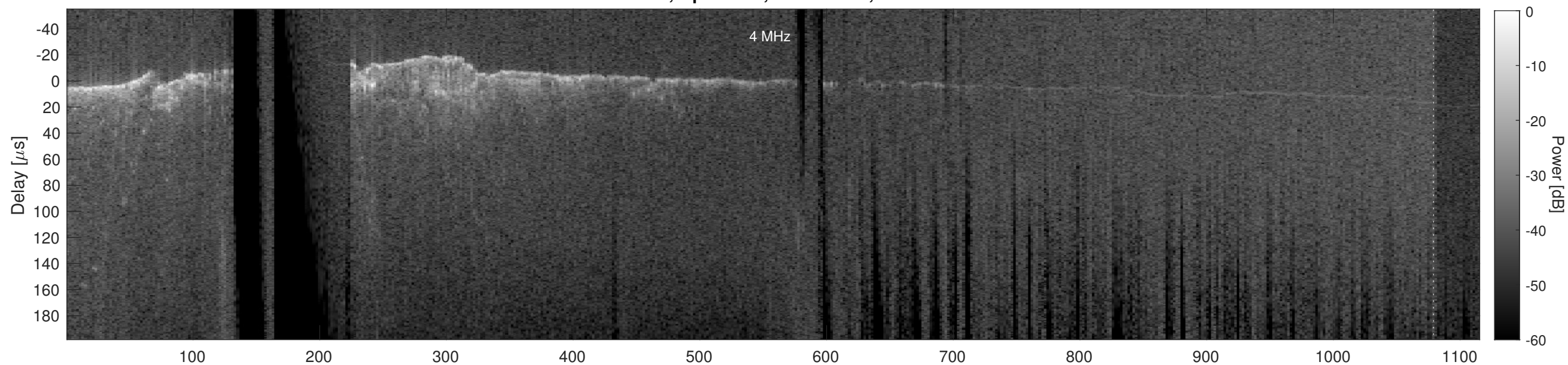
Orbit 2412, Cluttergram
