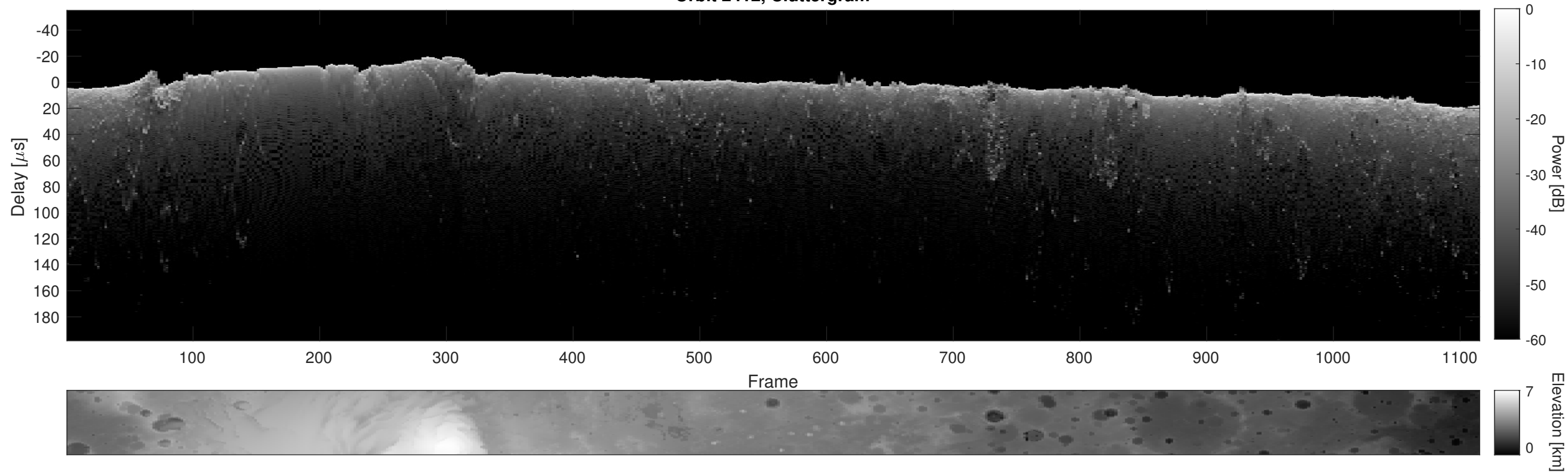
Orbit 2412, Cluttergram
