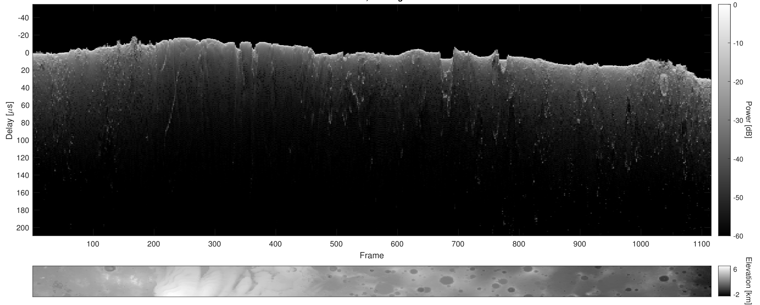
Orbit 2414, Cluttergram
