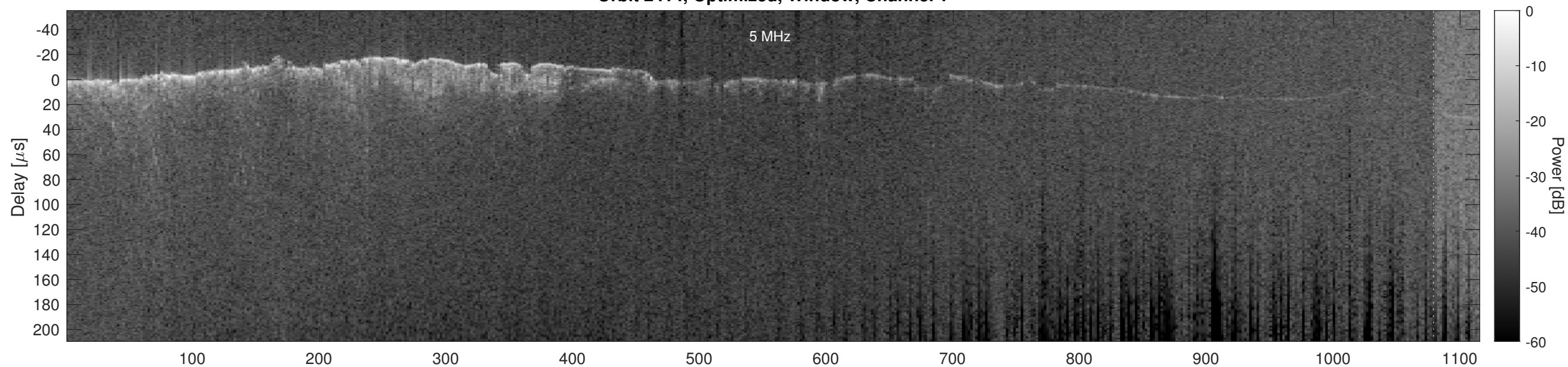
Orbit 2414, Optimized, Window, Channel 2
