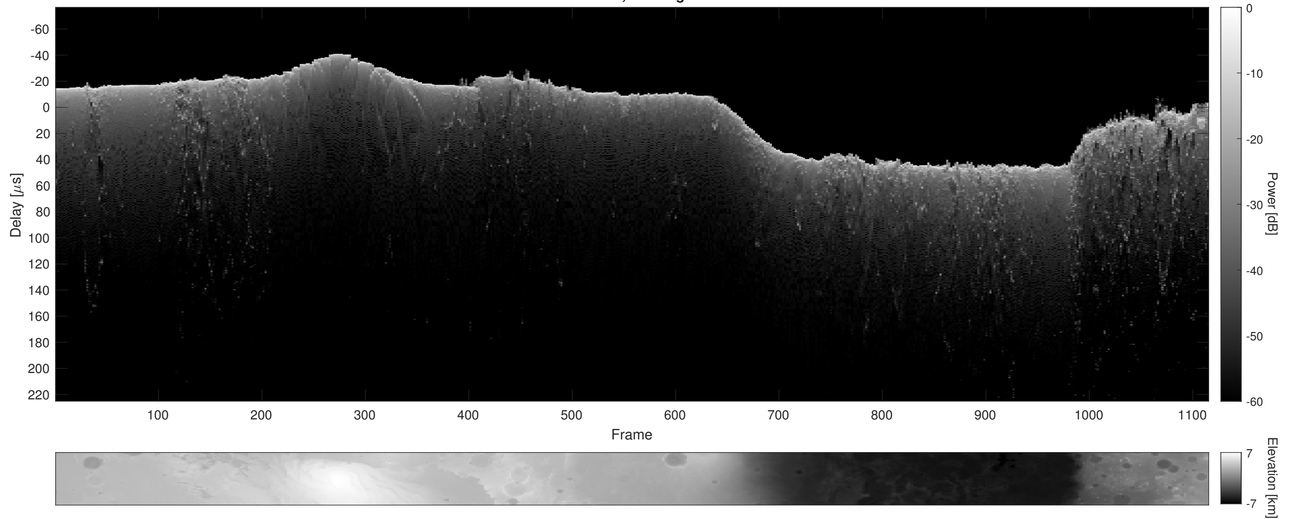
Orbit 2415, Cluttergram
