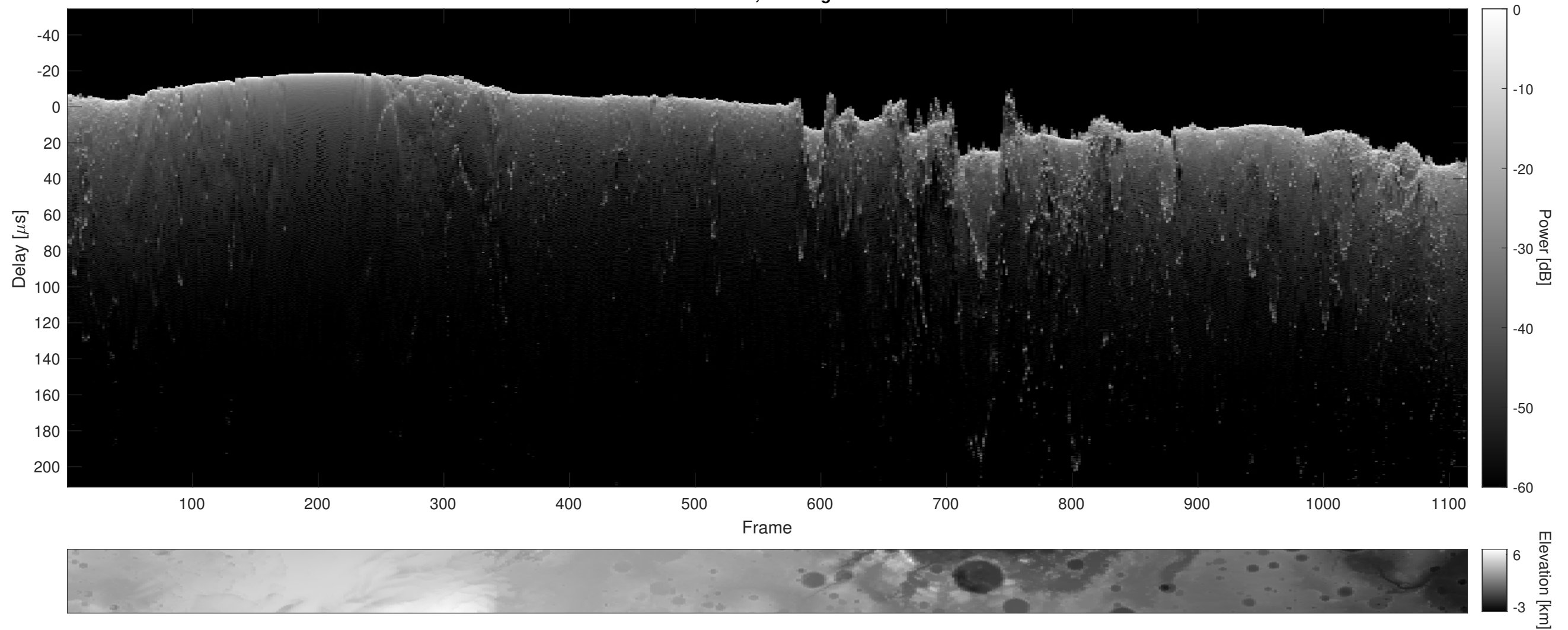
Orbit 2416, Cluttergram
