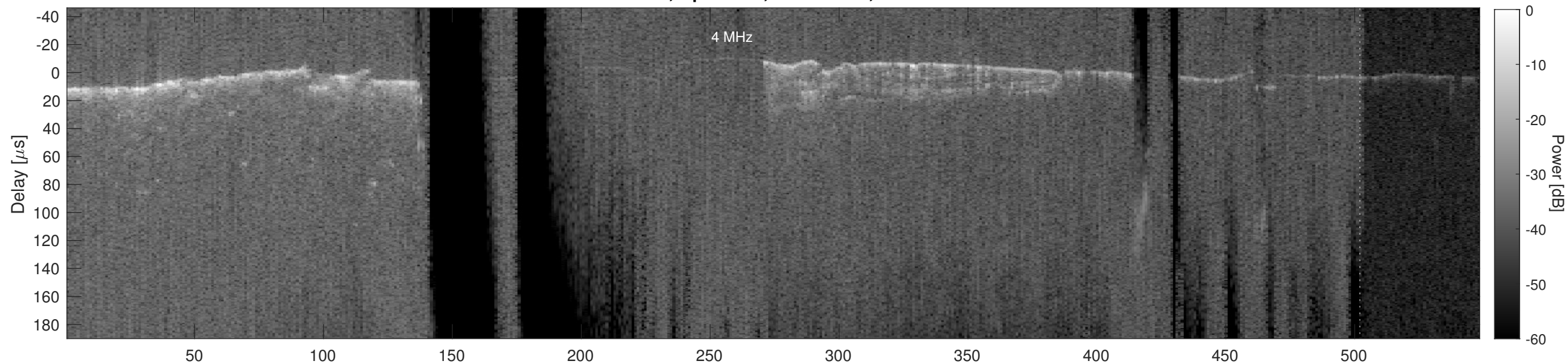
Orbit 2417, Cluttergram
