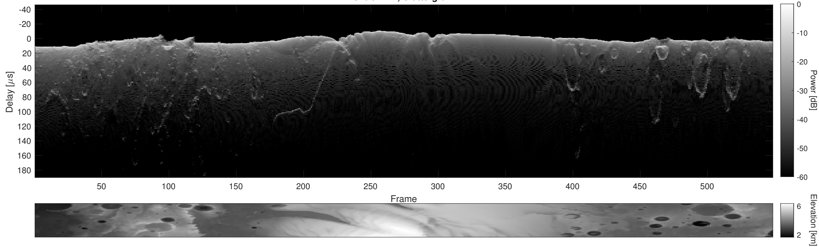
Orbit 2417, Cluttergram
