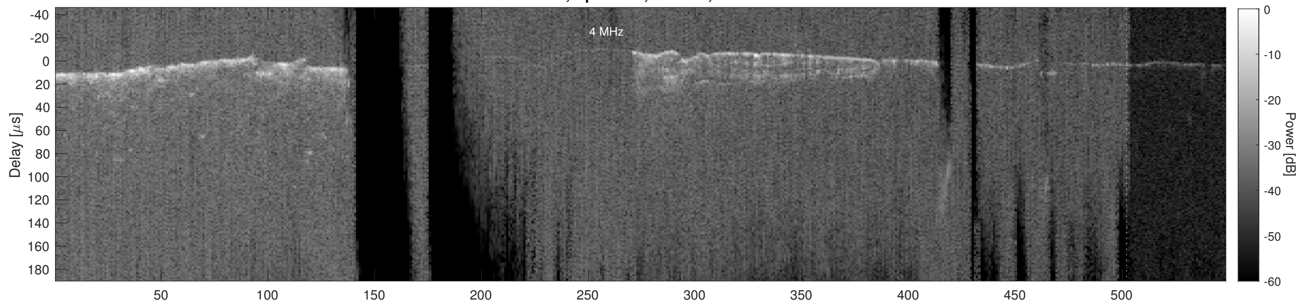
Orbit 2417, Cluttergram
