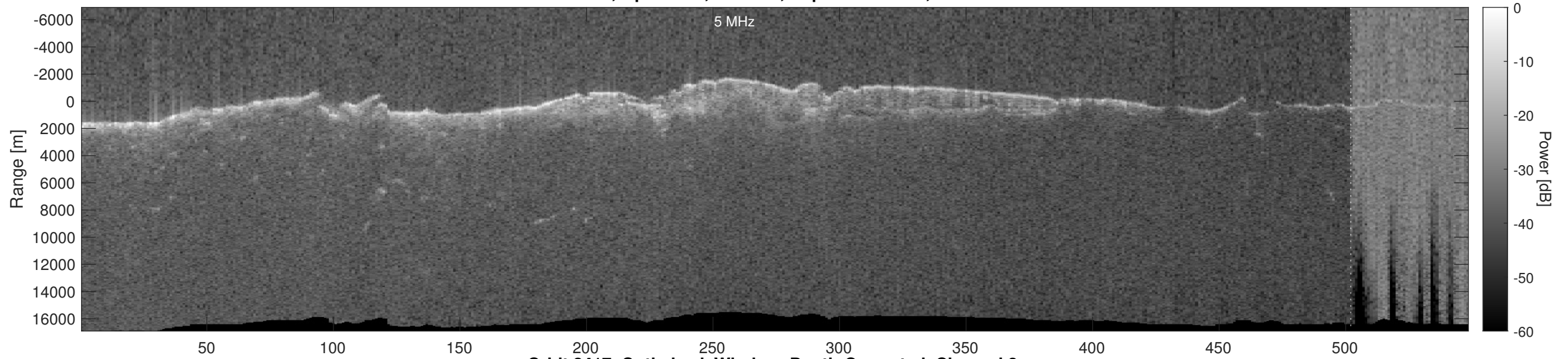
Orbit 2417, Optimized, Window, Depth-Corrected, Channel 2
