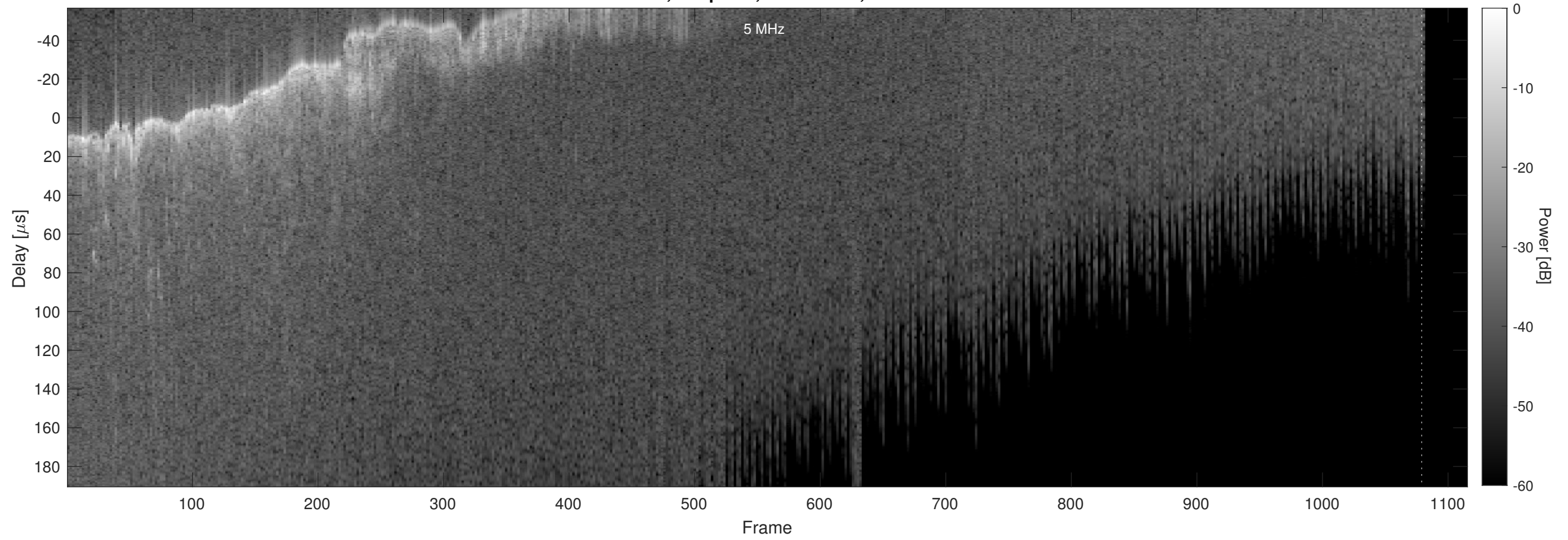
Orbit 2418, Chapman, No Window, Channel 2
