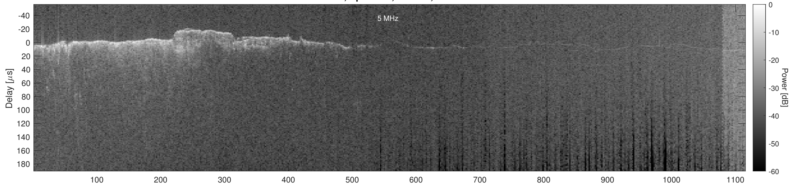
Orbit 2418, Optimized, Window, Channel 2
