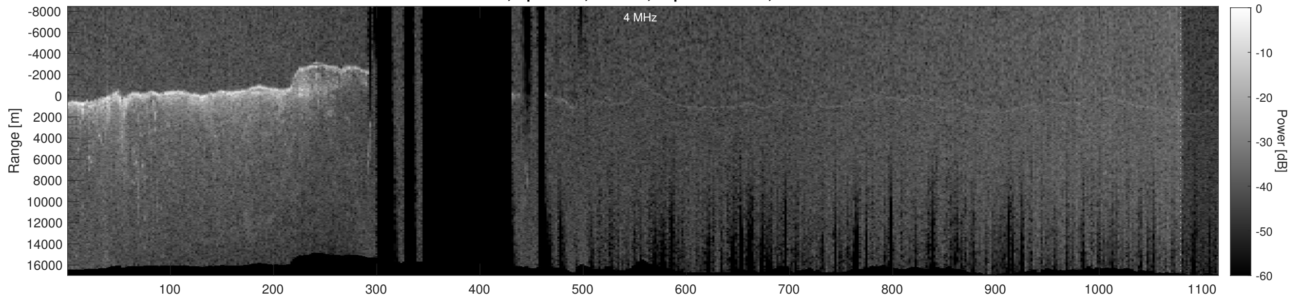
Orbit 2418, Depth-Corrected Cluttergram
