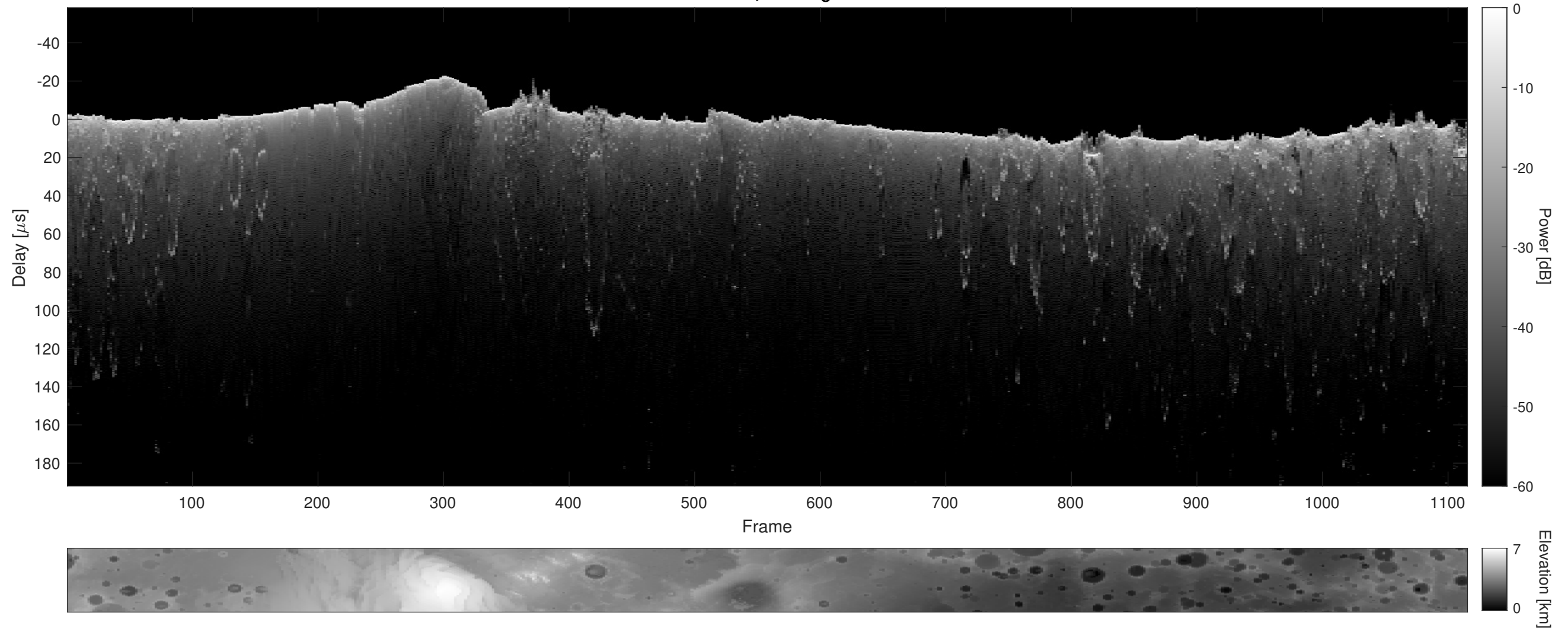
Orbit 2419, Cluttergram
