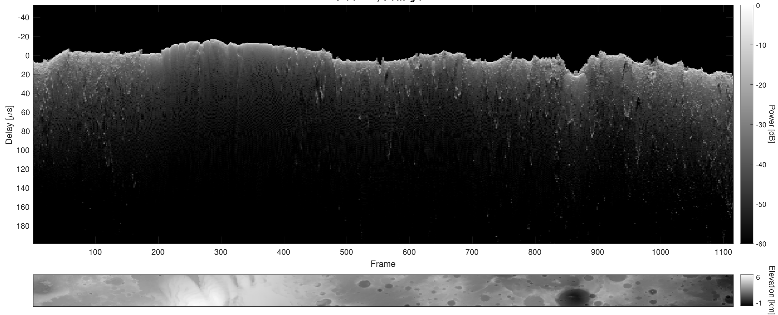
Orbit 2421, Cluttergram
