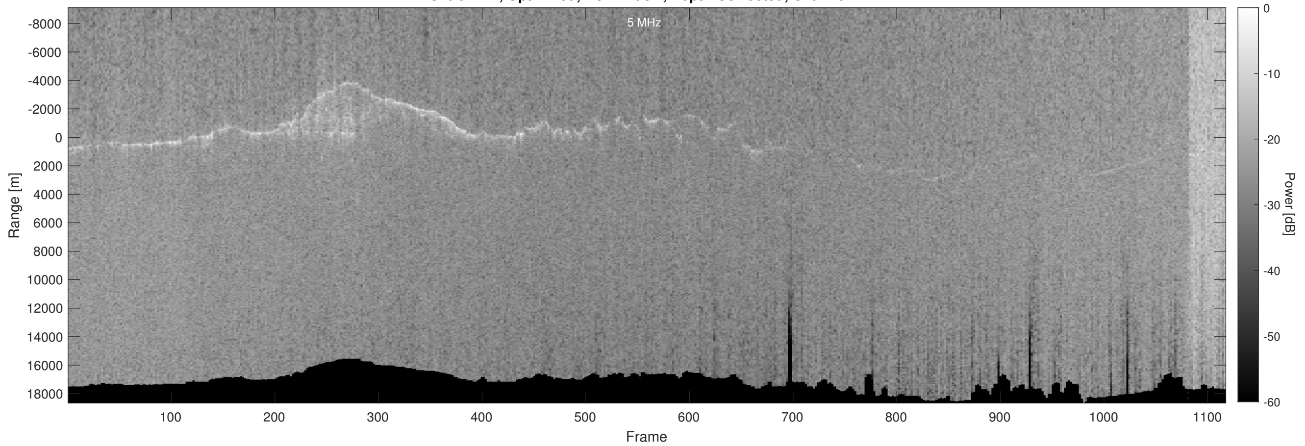
Orbit 2422, Optimized, No Window, Depth-Corrected, Channel 2
