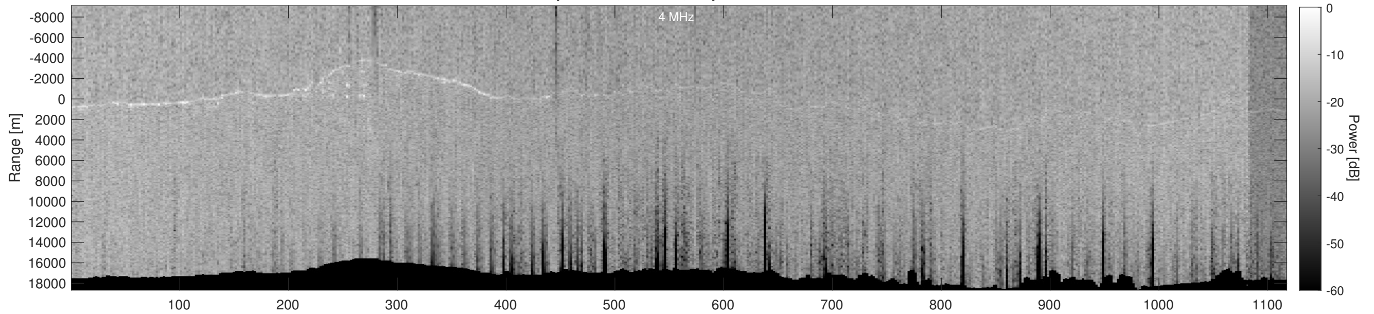
Orbit 2422, Depth-Corrected Cluttergram
