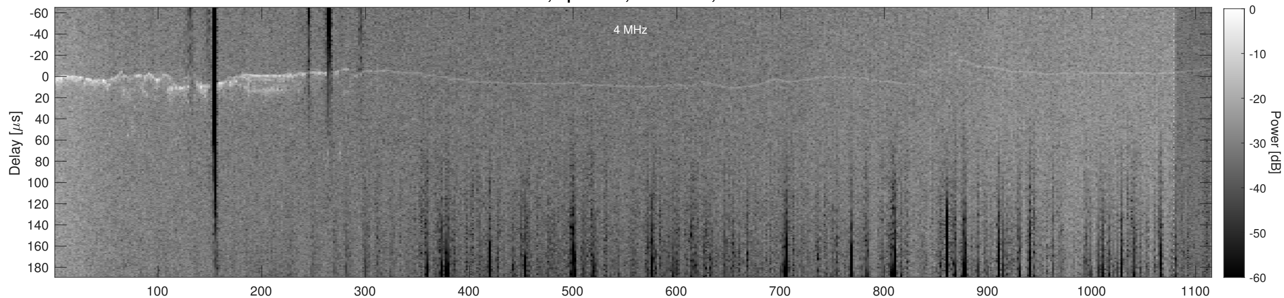
Orbit 2424, Cluttergram
