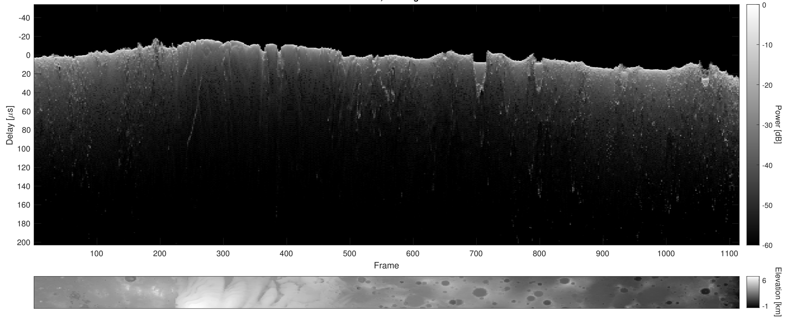
Orbit 2425, Cluttergram
