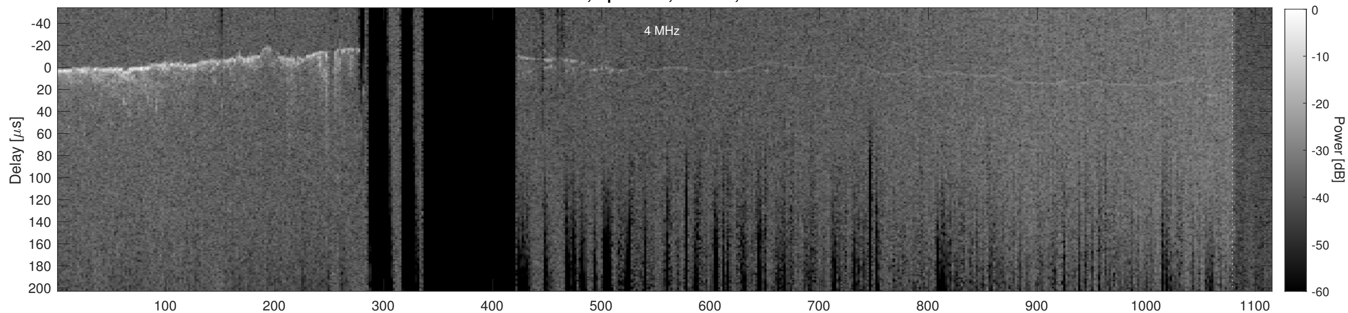
Orbit 2425, Cluttergram
