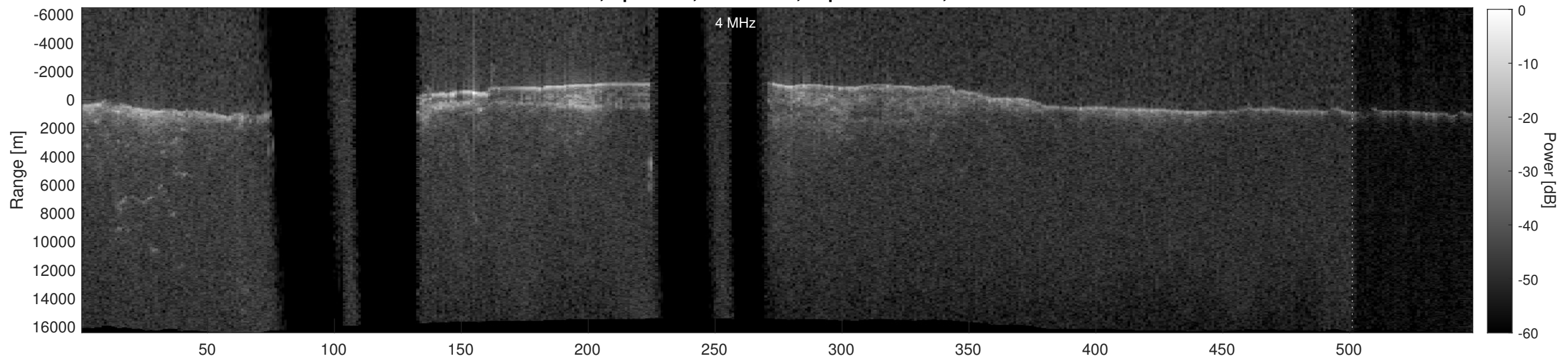
Orbit 2427, Depth-Corrected Cluttergram
