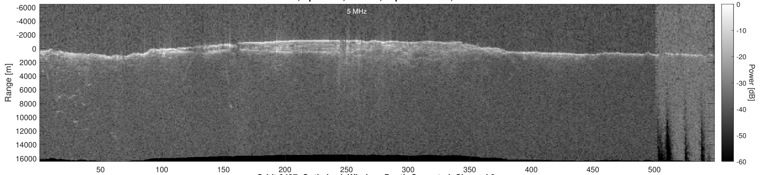
Orbit 2427, Optimized, Window, Depth-Corrected, Channel 2
