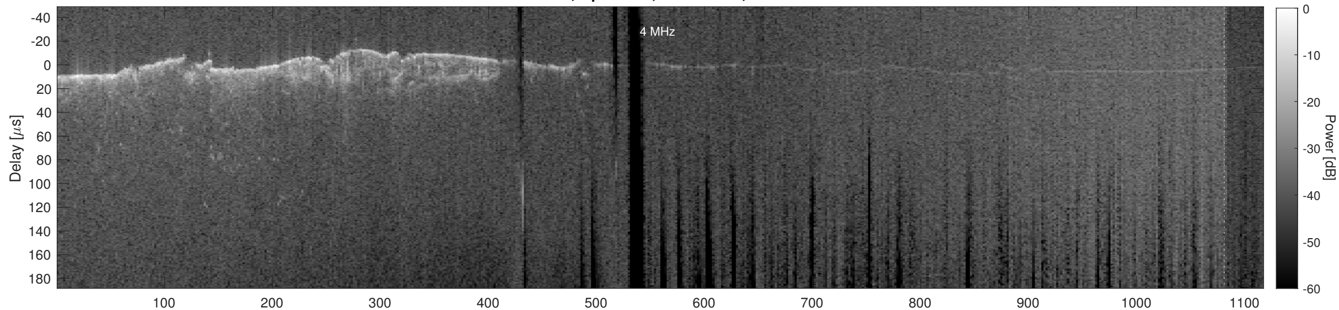
Orbit 2428, Cluttergram
