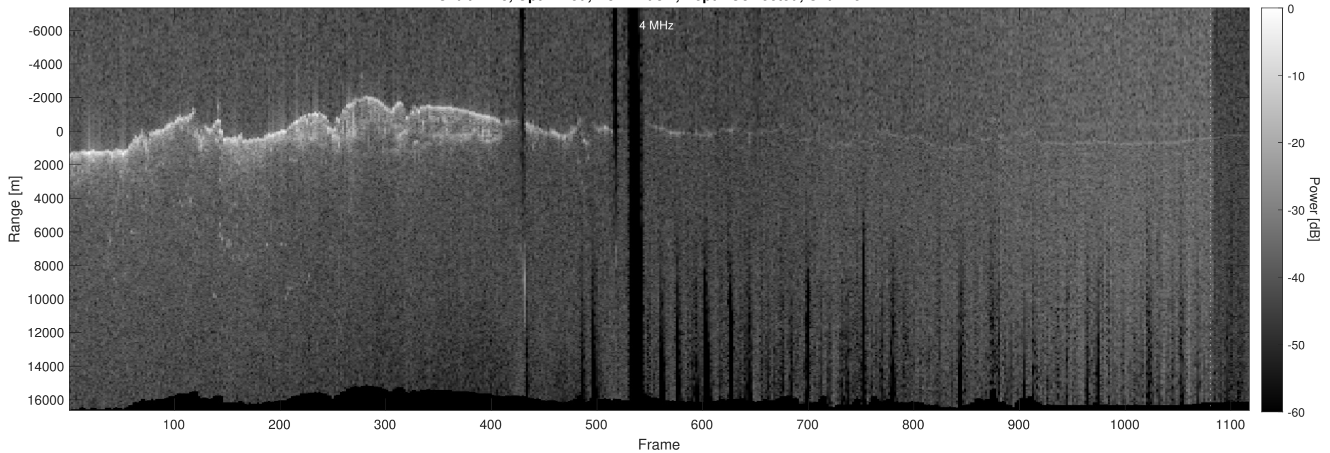
Orbit 2428, Optimized, No Window, Depth-Corrected, Channel 2
