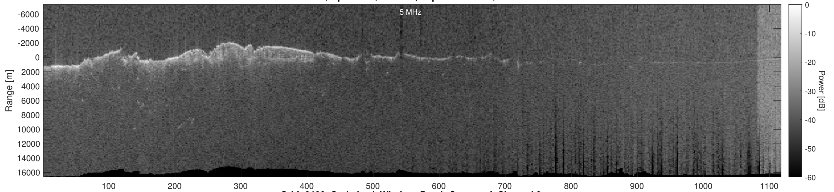
Orbit 2428, Optimized, Window, Depth-Corrected, Channel 2
