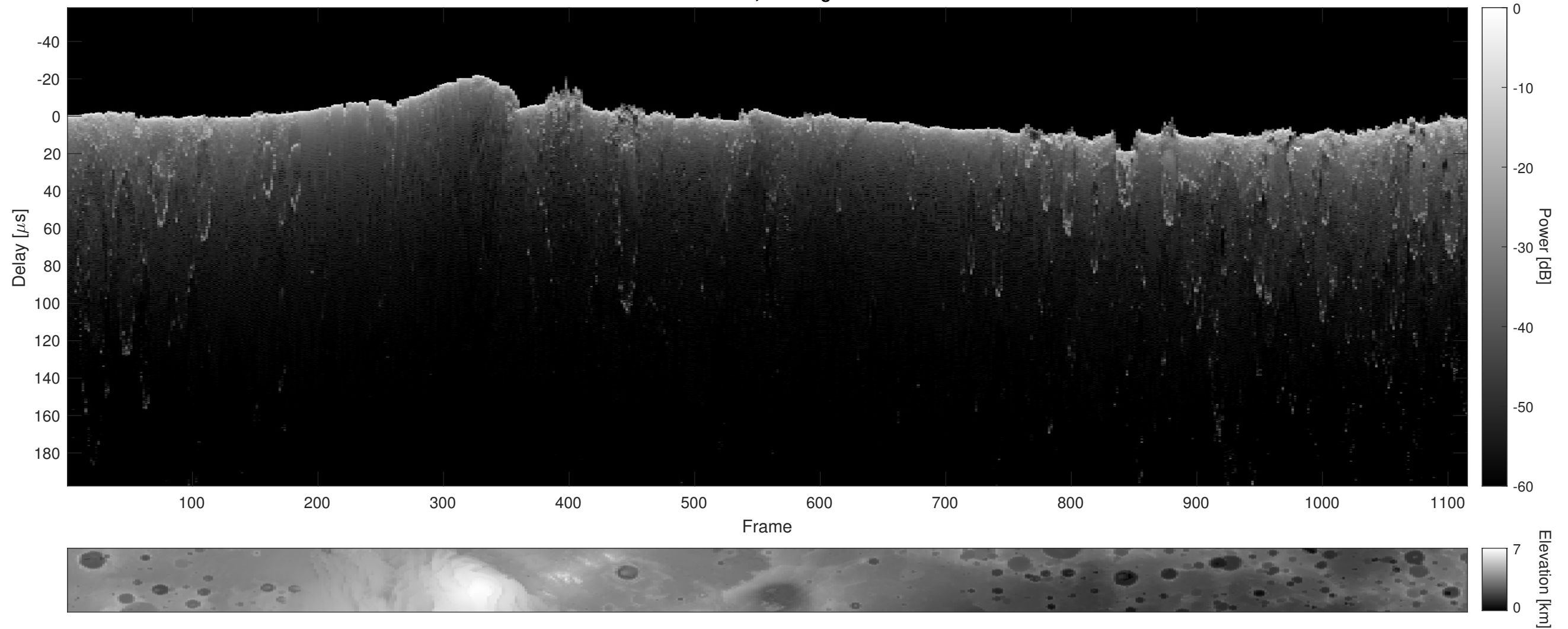
Orbit 2430, Cluttergram
