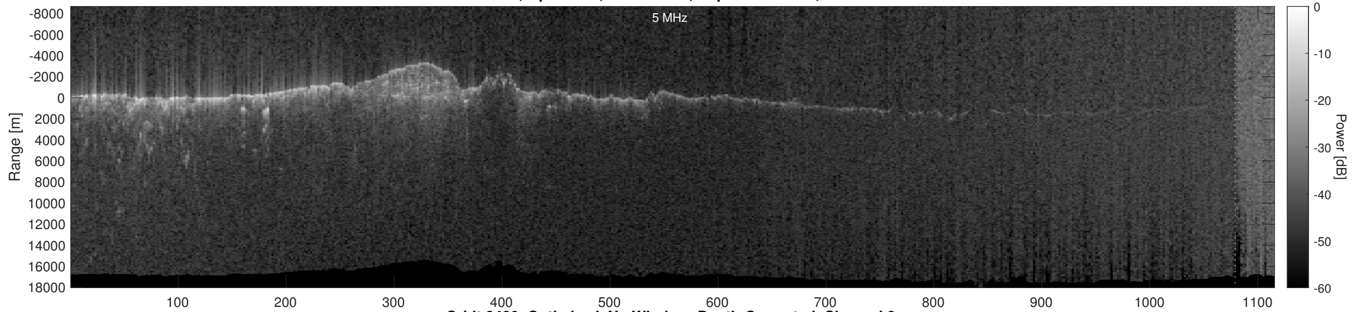
Orbit 2430, Optimized, No Window, Depth-Corrected, Channel 2
