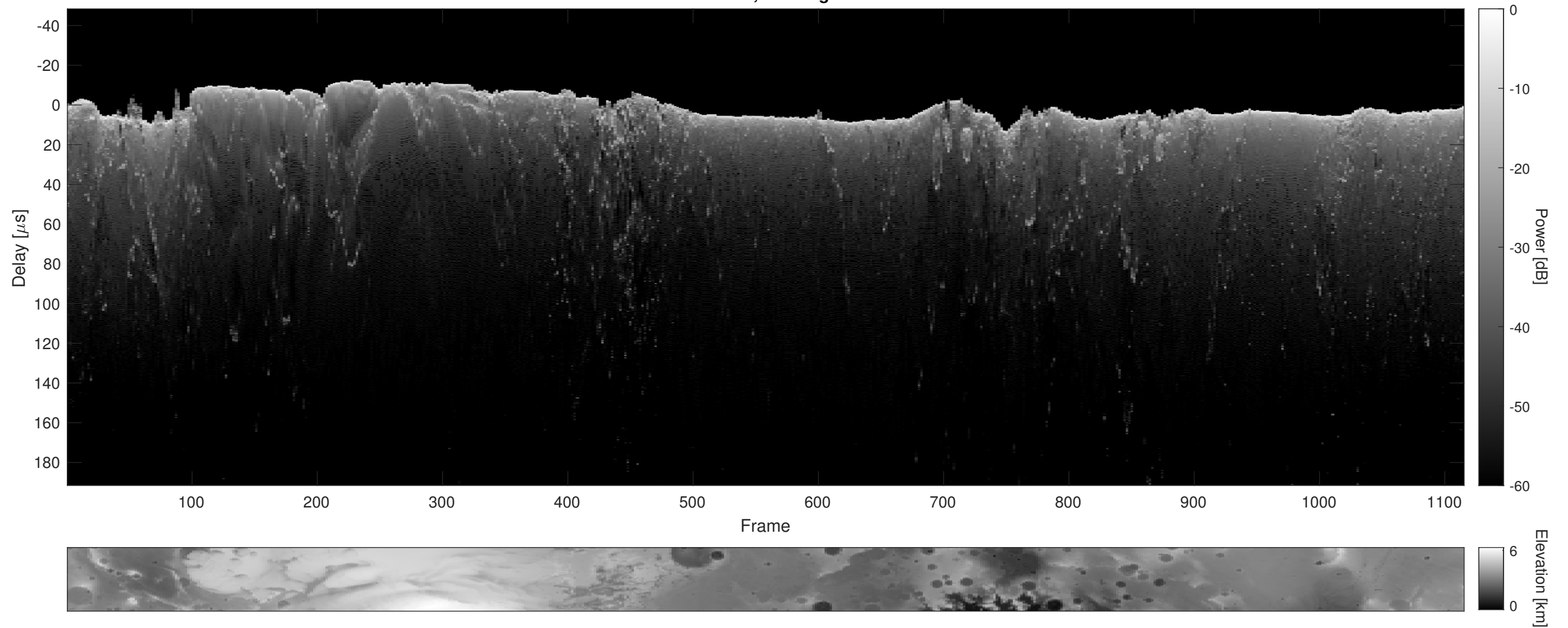
Orbit 2431, Cluttergram
