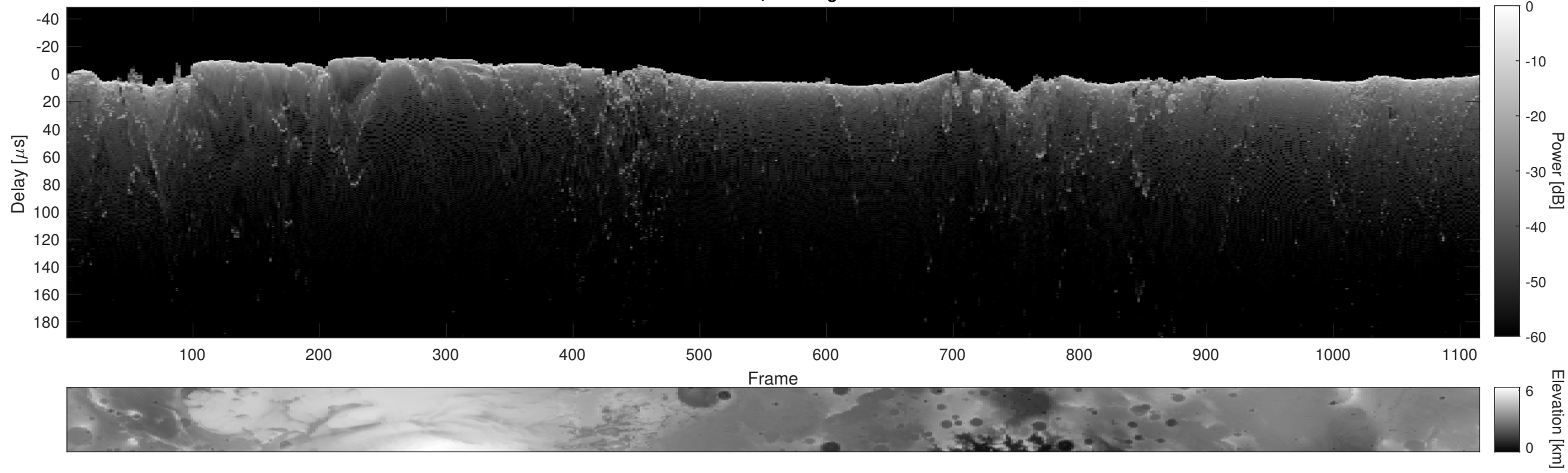
Orbit 2431, Cluttergram
