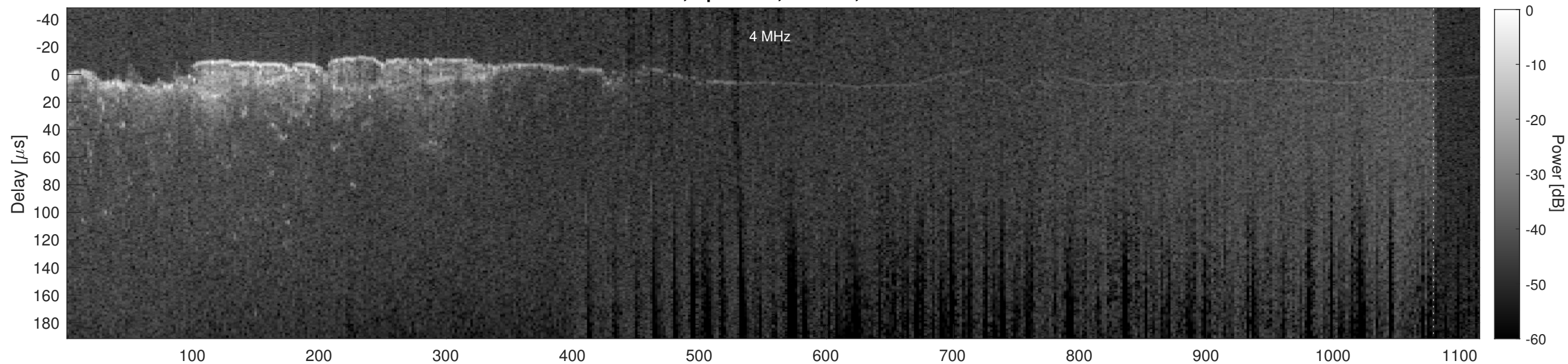
Orbit 2431, Cluttergram
