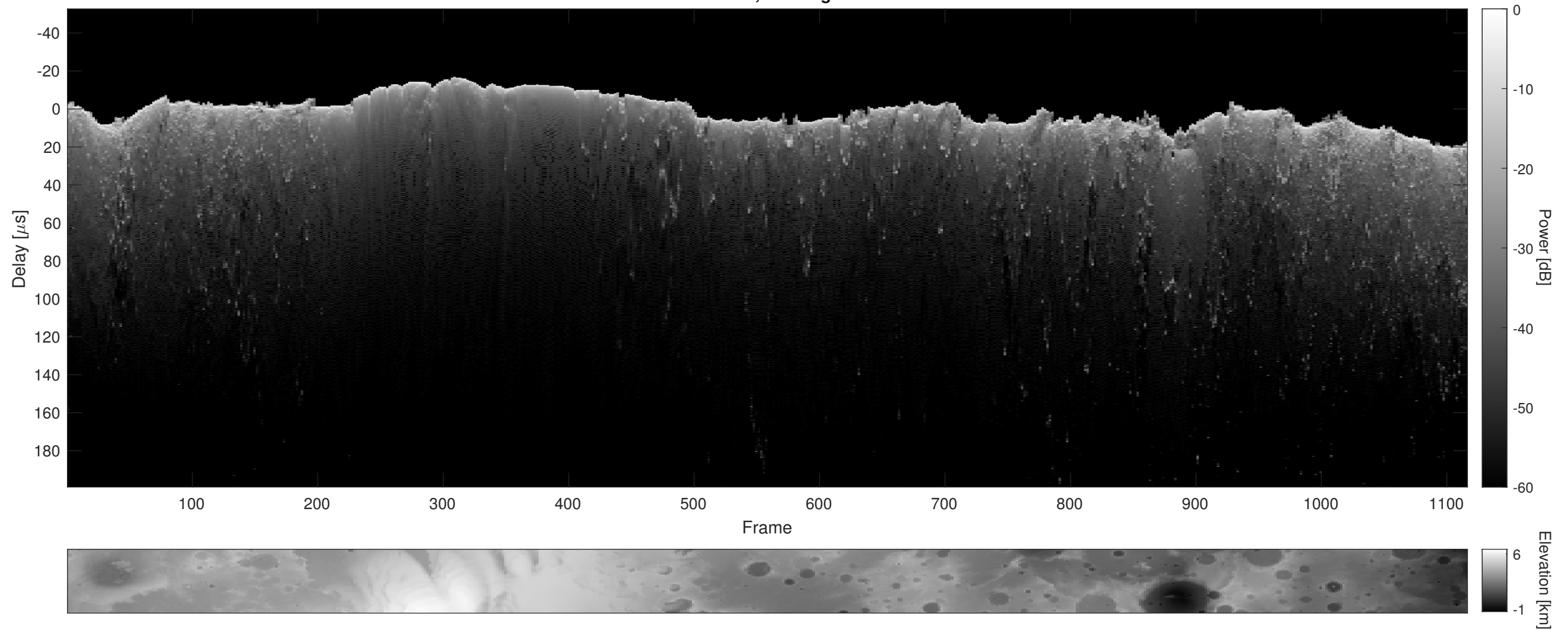
Orbit 2432, Cluttergram
