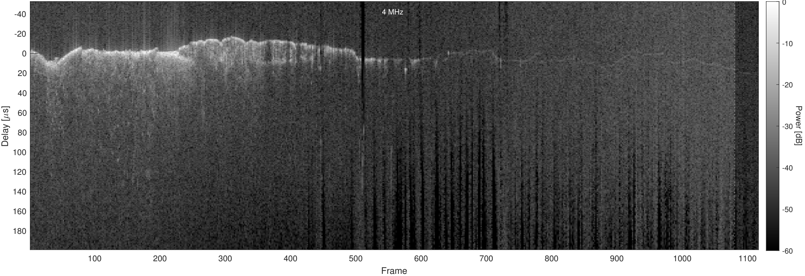
Orbit 2432, Optimized, No Window, Channel 2
