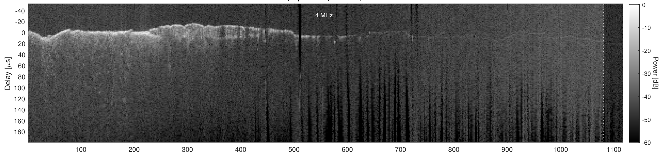
Orbit 2432, Cluttergram
