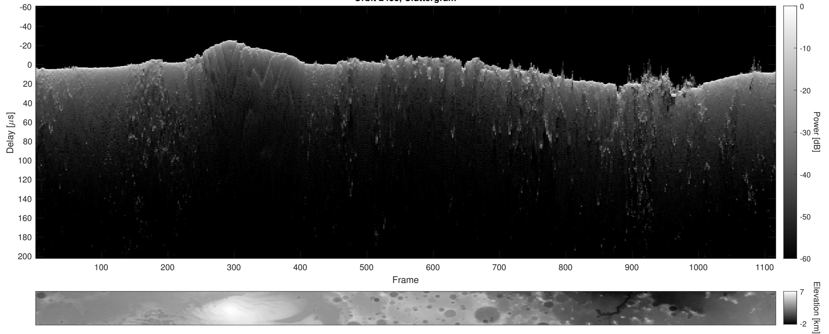
Orbit 2433, Cluttergram
