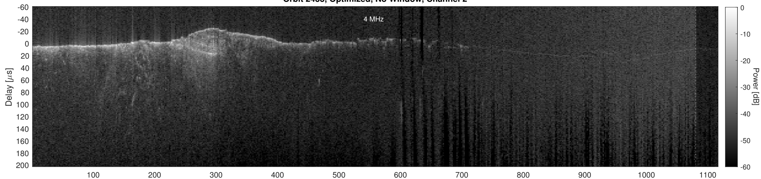
Orbit 2433, Cluttergram
