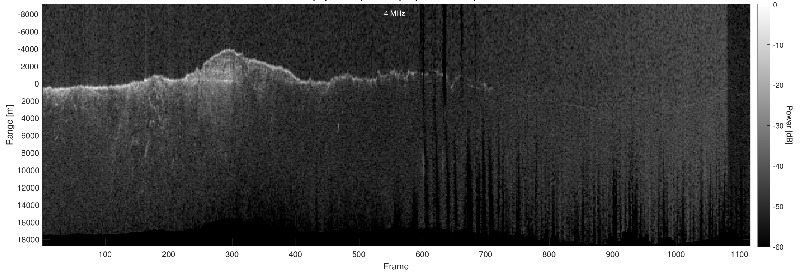
Orbit 2433, Optimized, Window, Depth-Corrected, Channel 2
