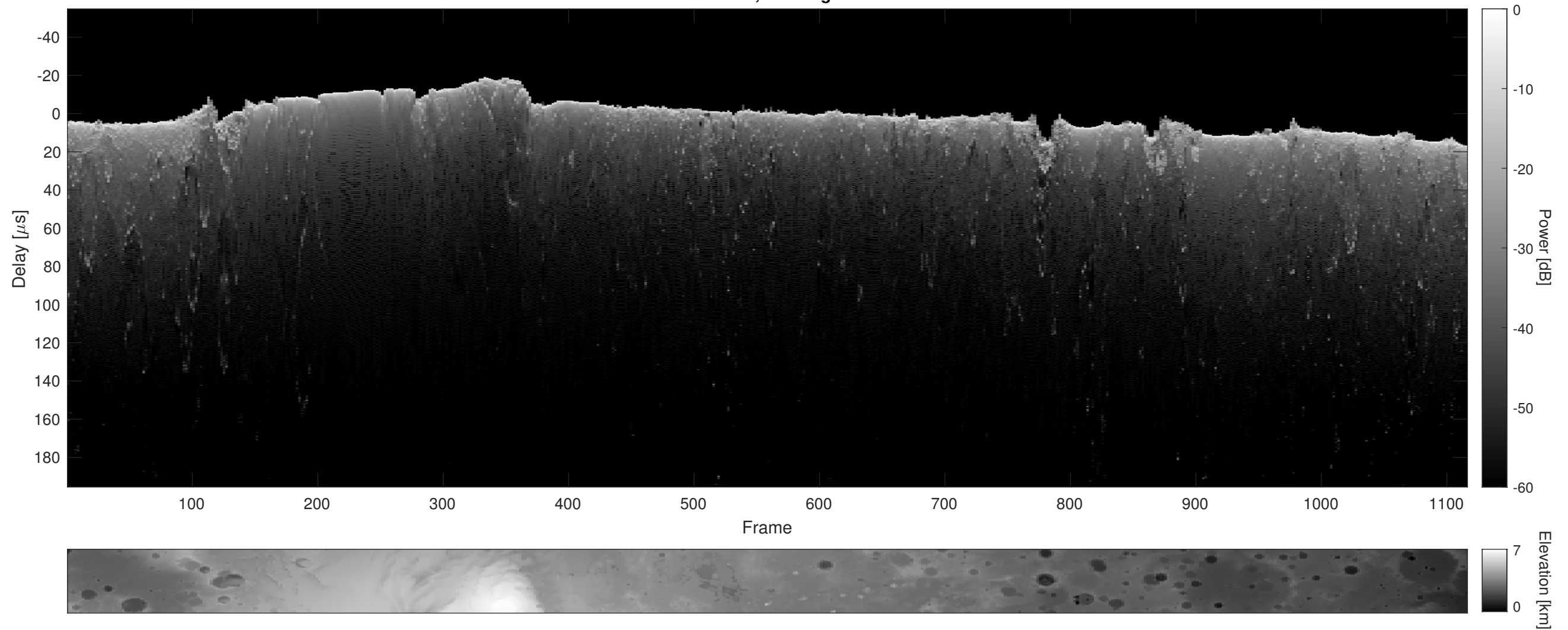
Orbit 2434, Cluttergram
