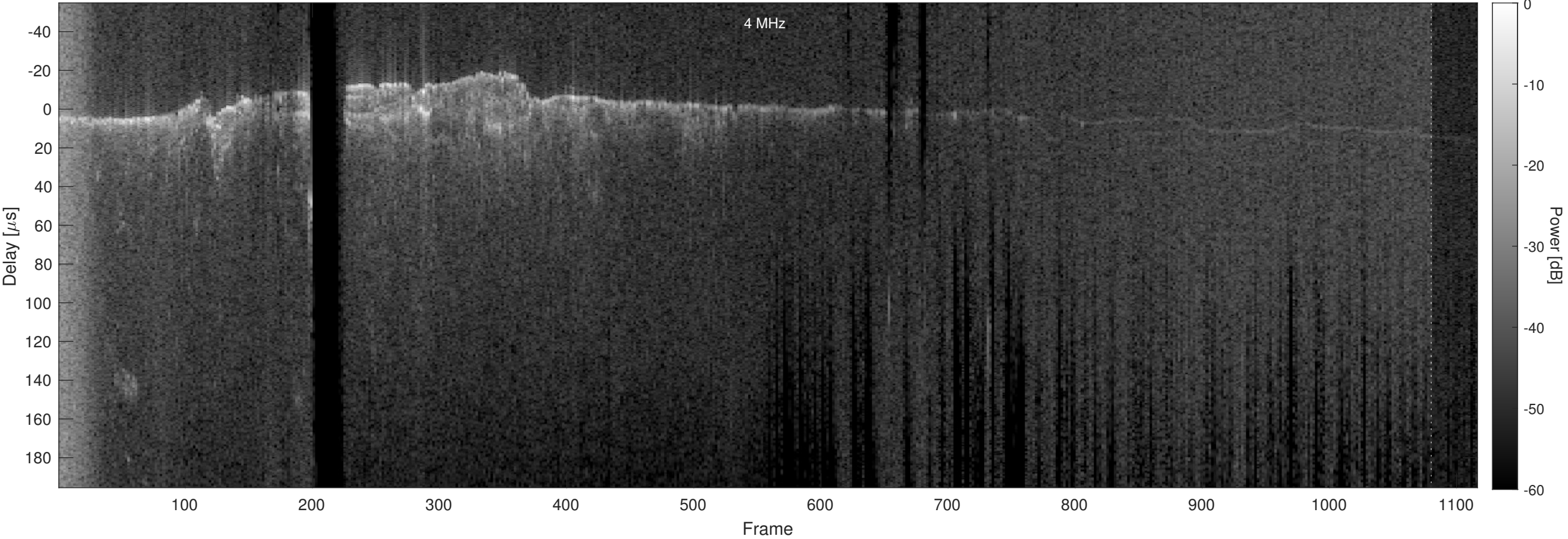
Orbit 2434, Optimized, No Window, Channel 2
